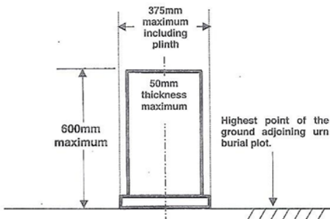
Figure 4: URN BURIAL PLOT HEADSTONE AND CROSS OVERALL DIMENSIONS
