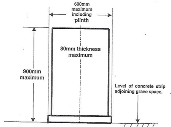
Figure 3: GRAVE SPACE HEADSTONE and CROSS OVERALL DIMENSIONS
