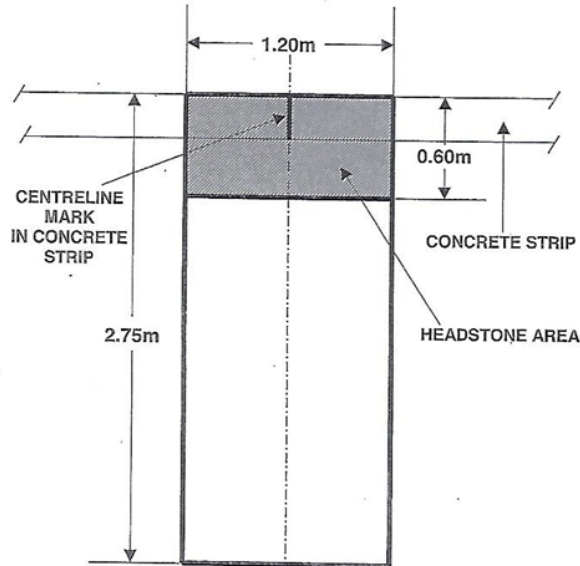
Figure 1: GRAVE SPACE DIMENSIONS
